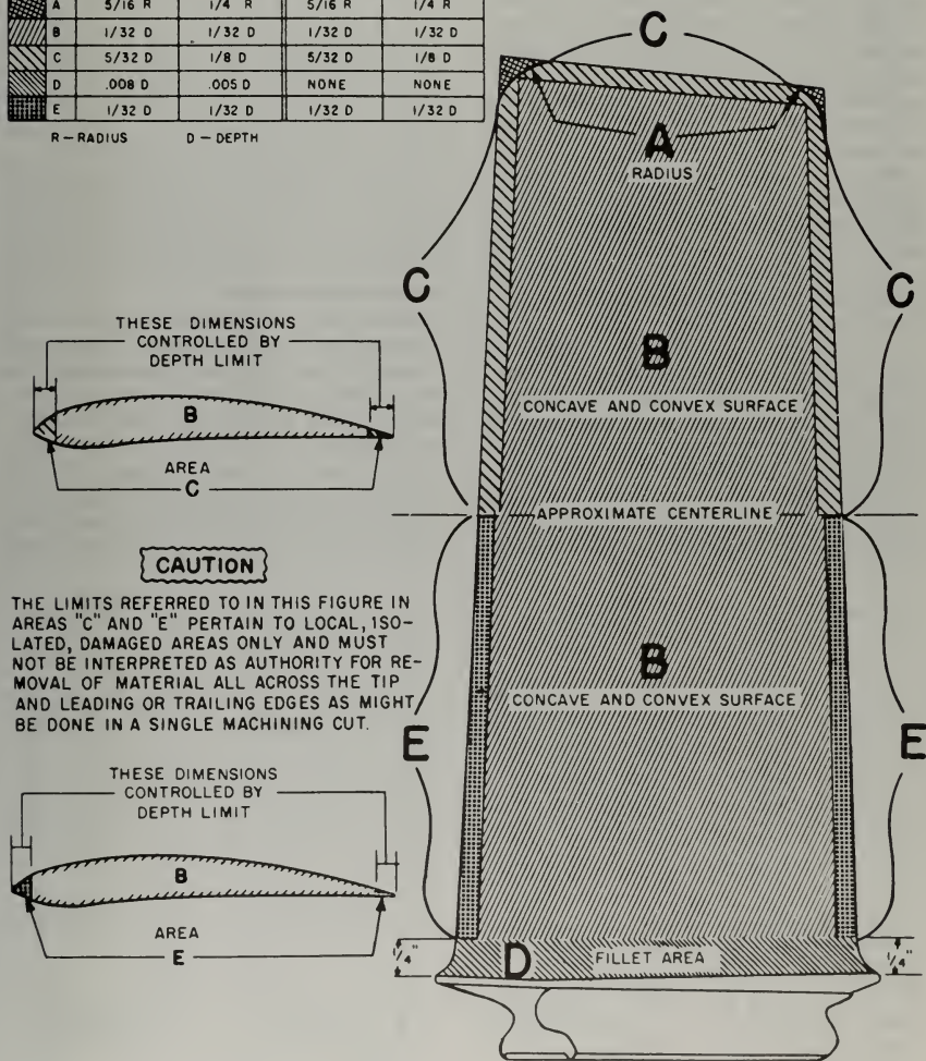
FIGURE 10-54. Typical compressor blade repair limits.
